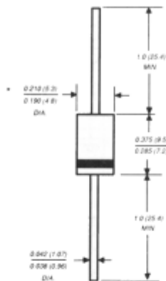
Case Style 1.5KE
