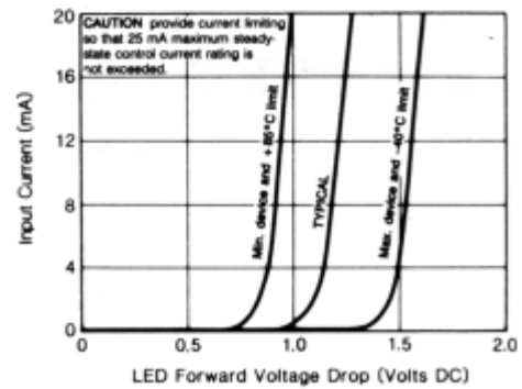
Figure 6. Input Characteristics (Current Controlled)
