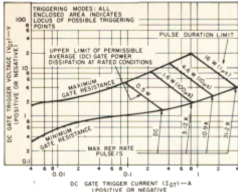
Fig. 7 - Gate trigger characteristics and limiting conditions for permissible gate trigger pulses.
